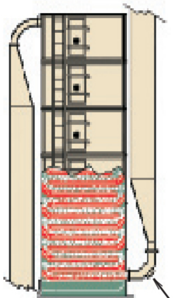
INSIDE VIEW OF TOWER DRIER Shown With Optional Magnetic Elbow
